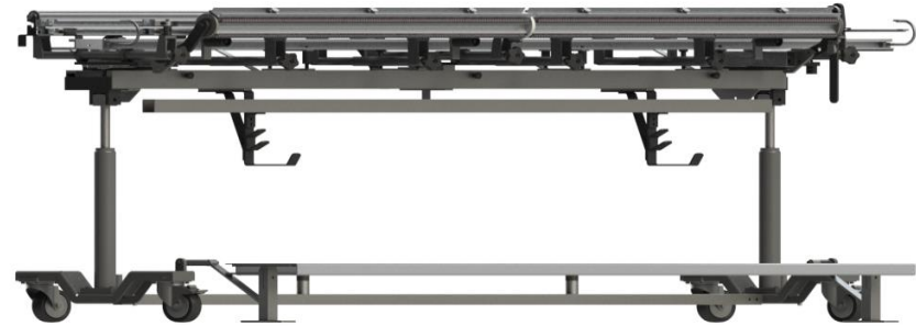
STANDARD MODEL
